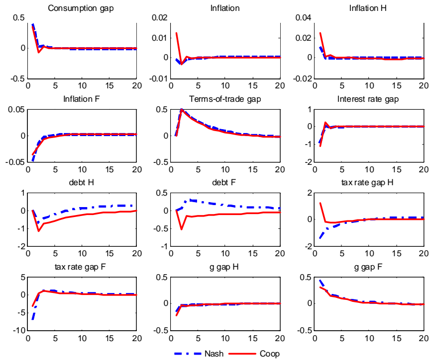
Figure 4: Responses to a 1% negative technology shock at H
